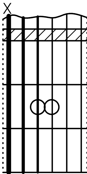
A sus2
